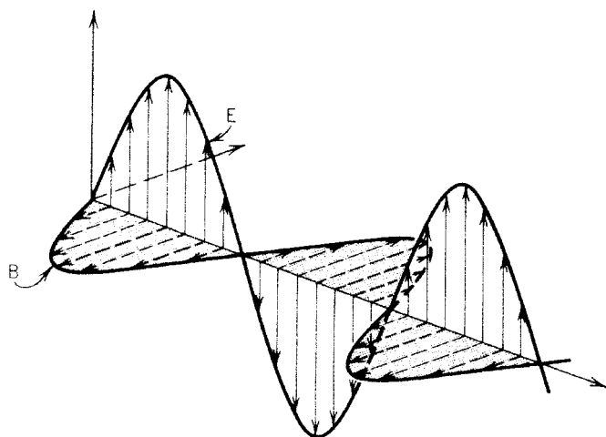
FIGURE 1.6 An electromagnetic wave showing the coupled electric (E) and magnetic (B) fields as they oscillate in their motion through space.
