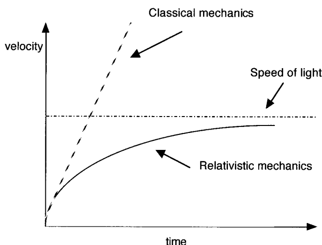
FIGURE 1.1 A graph of velocity versus time, representing acceleration, in Newtonian mechanics and in relativistic mechanics. Relativistic and Newtonian mechanics predict the same values for acceleration at low velocities. At high velocities, relativistic mechanics predicts smaller and smaller values for acceleration, contrary to Newtonian mechanics.
